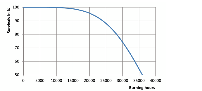
SON(-T) PIA Plus 150W 250W 400W Life Expectancy Diagram
