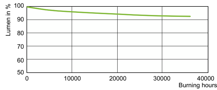
Lumen Maintenance Diagram - MST SON-T PIA Plus 250W E E40 1SL/12
