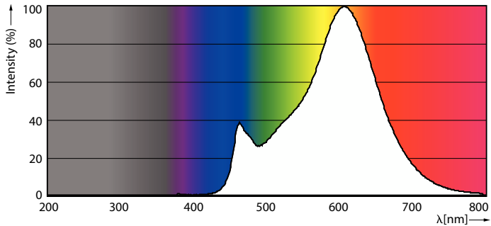
Spectral Power Distribution Colour - CorePro LEDLusterND4.3-40W E27 827P45CLG
