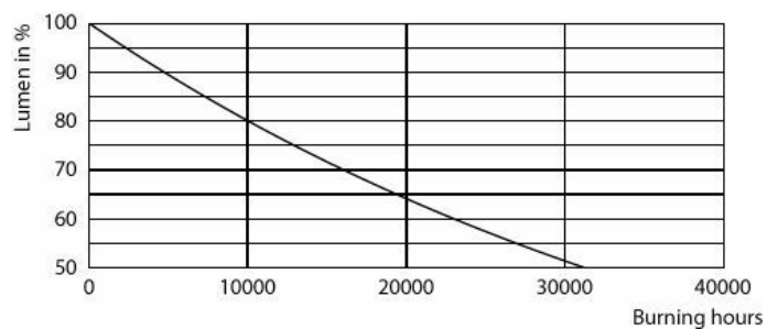
Lumen Maintenance Diagram - MZD LED 25W E27 827 P45 FR ND 1CT/10
