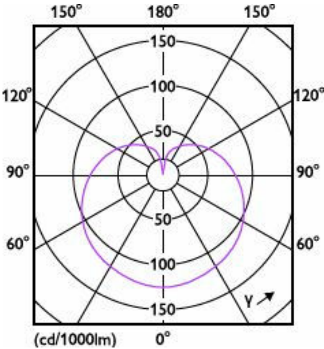
Light Distribution Diagram - MZD LED 25W E27 827 P45 FR ND 1CT/10
