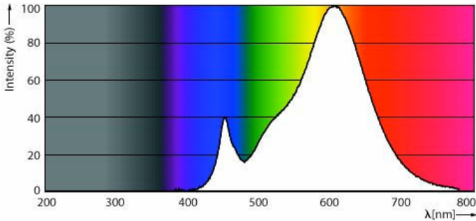
Spectral Power Distribution Colour - MZD LED 25W E27 827 P45 FR ND 1CT/10
