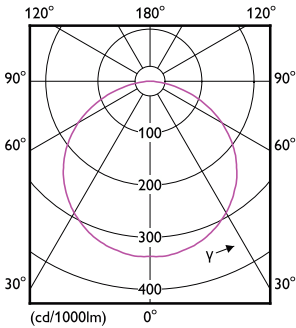
Light Distribution Diagram - MAS LEDstrip 8.3W965 950LM/M 5M
