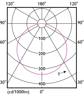
Light Distribution Diagram - MAS LEDstrip 4.3W940 500LM/M 5M
