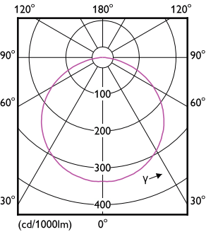
Light Distribution Diagram - MAS LEDstrip 4.3W930 475LM/M 5M
