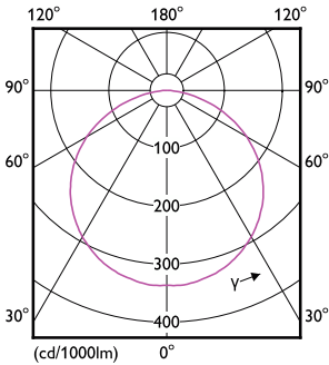
Light Distribution Diagram - MAS LEDstrip 4.3W927 475LM/M 5M
