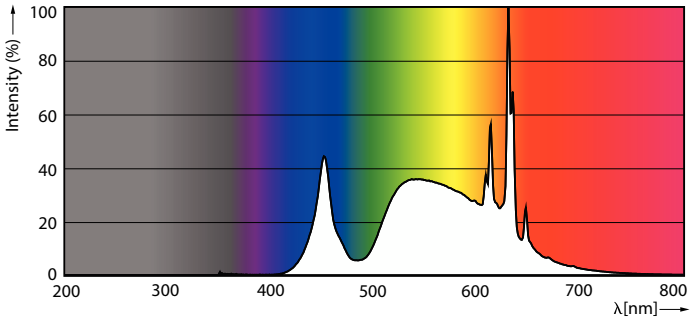
Spectral Power Distribution Colour - MAS LEDBulbND2.3-40W E27 840 A60 CL G UE
