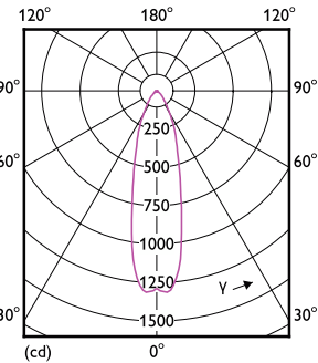
Light Distribution Diagram - MAS LEDspot VLE D 6-50W 940 PAR20 25D
