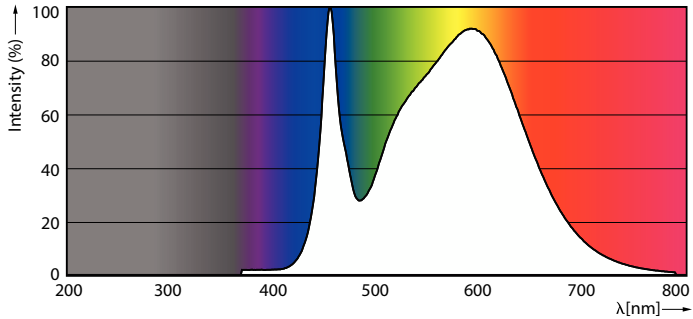
Spectral Power Distribution Colour - LED D2D 60W A60 E27 CW FR ND SRT4
