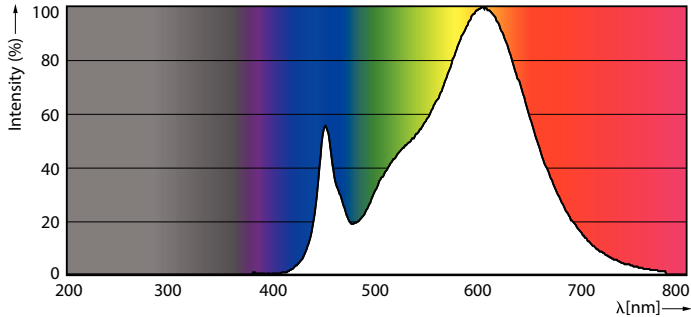
Spectral Power Distribution Colour - TForce LED HPL ND 57-42W E27 830
