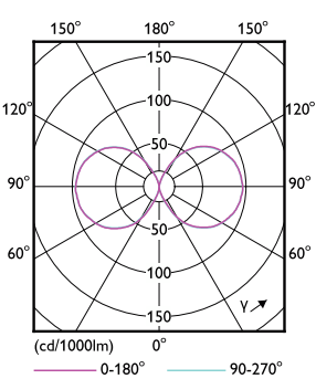
Light Distribution Diagram - TForce LED HPL ND 57-42W E27 830
