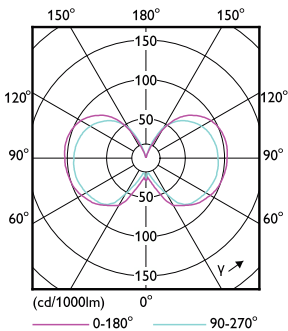
Light Distribution Diagram - LED classic 60W G95 E27 CW FR ND 1PF/4
