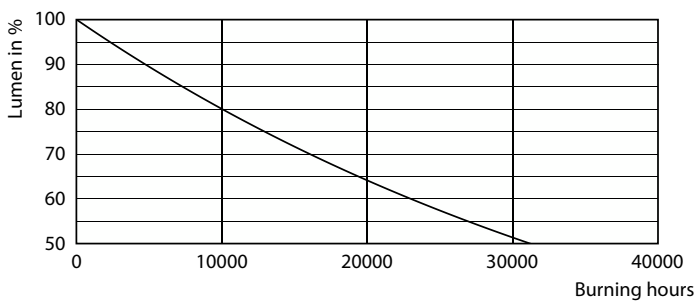
Lumen Maintenance Diagram - LED classic 60W G95 E27 WW FR ND RFSRT4
