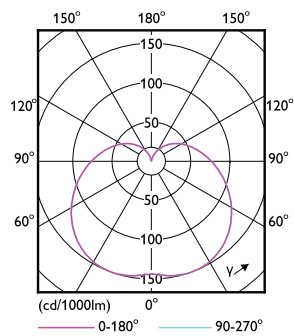
Light Distribution Diagram - Corepro LEDBulbND 3.2Klm 30W830 E27T100
