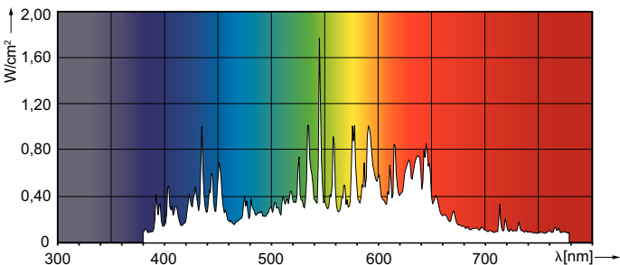
Spectral Power Distribution Colour - MASTERCoulour CDM-T MW eco 230W/842 E40
