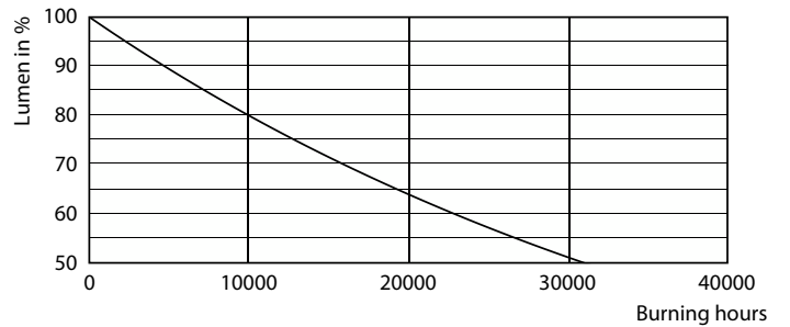
Lumen Maintenance Diagram - LED 25W T25 E14 WW FR ND 1SRT4
