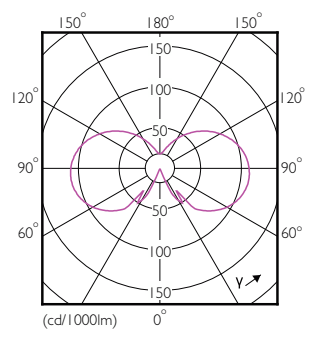
Light Distribution Diagram - CorePro LEDCandleND4.3-40W E14 827B35FRG
