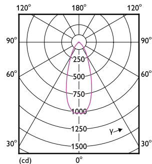
Light Distribution Diagram - CorePro LED spot ND 7-50W MR16 830 36D
