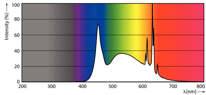
Spectral Power Distribution Colour - MAS LED spot VLE D 5.5-80W GU10 965 36D
