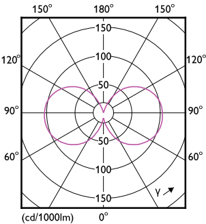
Light Distribution Diagram - LED classic 75W G120 E27 WW FR ND SRT4
