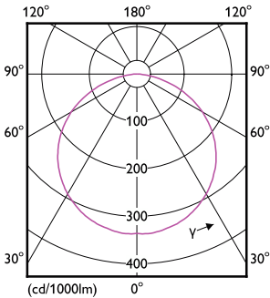
Light Distribution Diagram - CorePro LEDstrip 9.2W865 1180LM/M 5M
