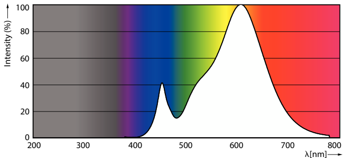
Spectral Power Distribution Colour - CorePro LED spot ND 2.9-20W MR16 827 36D
