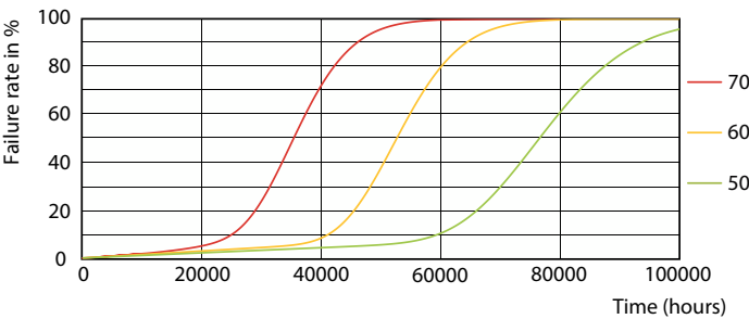
LEDtube-75K-5070-FailureRate-LED
