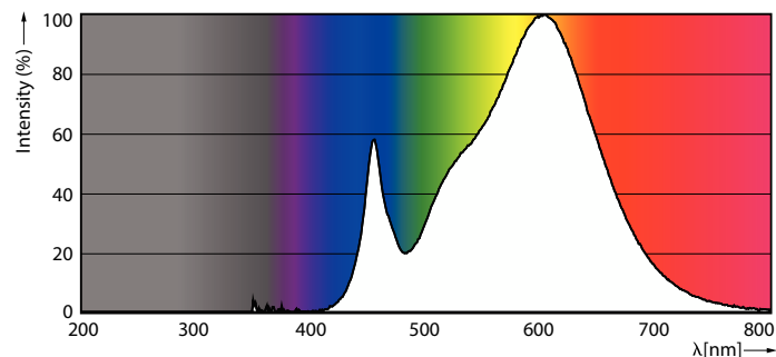
Spectral Power Distribution Colour - Corepro LEDspot 670lm GU10 830 60D
