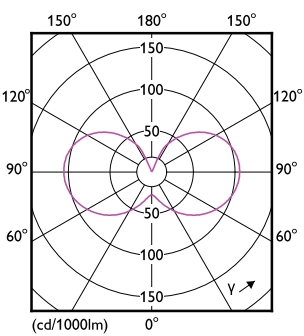
Light Distribution Diagram - CorePro LEDLusterND6.5-60W P45 E14827FRG
