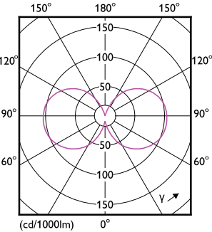
Light Distribution Diagram - LED classic 75W G120 E27 CW FR ND 1PF/4
