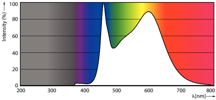
Spectral Power Distribution Colour - LED classic 75W G120 E27 CW FR ND 1PF/4
