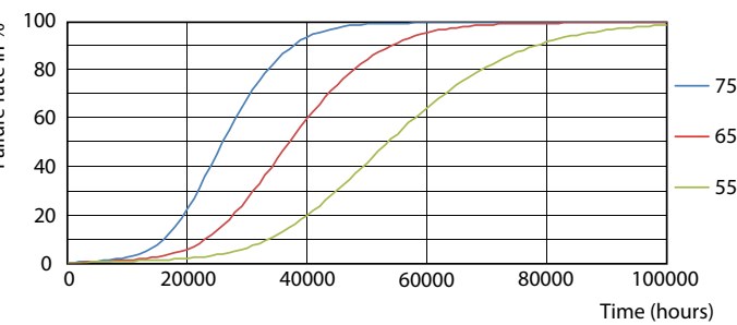
FailureRate
