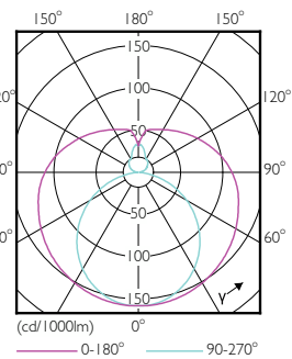
Light Distribution Diagram - CorePro LEDtube UN 1200mm HO 18W830 T8
