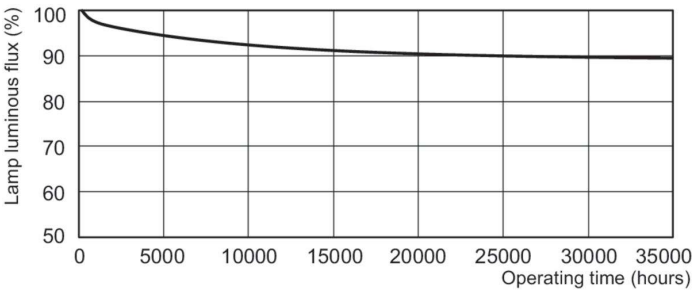
Lumen Maintenance Diagram - MASTER TL5 HE 14W/830 1SL/20
