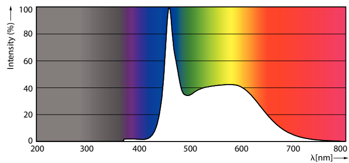
Spectral Power Distribution Colour - LED classic 60W G93 E27 CDL FR ND 1PF/4
