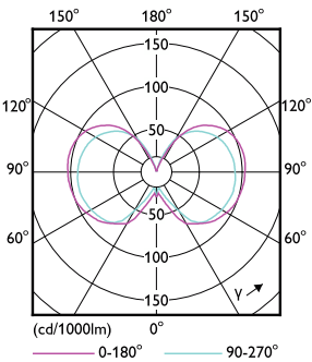
Light Distribution Diagram - LED classic 60W G93 E27 CDL FR ND 1PF/4
