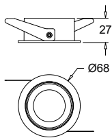
Cut out: Ø60 TITLE :RS378Z M55 D60 R-R FX
