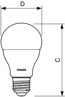
CorePro LEDbulb ND 10-75W A60 E27 840
