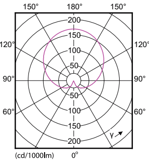
CorePro LEDbulb ND 7.5-60W A60
