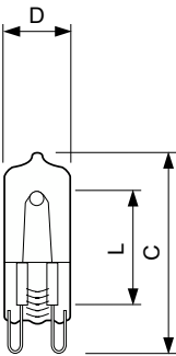
Halogen MV Click 19.0W G9 230V CL 1CT
