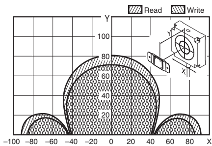
V680-HS52 (embedded in non-metallic material) & V680-D1KP66MT (mounted on metallic surface: steel)
