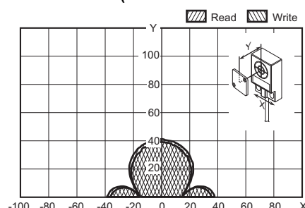
V680-HS61 (mounted on non-metallic material) & V680-D1KP66T (mounted on non-metallic material)
