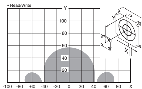
V680-HS63 (mounted on non-metallic material) & V680S-D8KF68 (Tag direction: Vertical)
