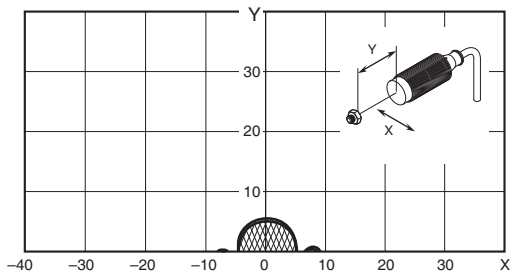
High-temperature Type 1-kbyte Memory RF Tags V680-HS65 (with metal on back surface) & V680-D1KP58HTN
