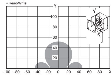
V680-HS52 (embedded in non-metallic material) & V680S-D8KF67M (mounted on metallic surface: steel)
