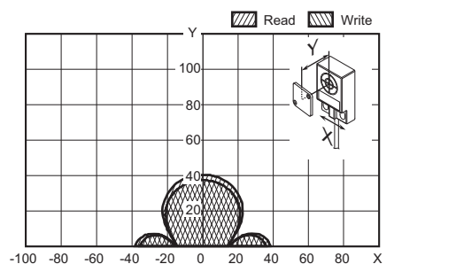
V680-HS61 (mounted on non-metallic material) & V680-D1KP66T (mounted on non-metallic material)
