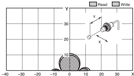
V680-HS61 (mounted on non-metallic material) & V680-D1KP52MT (embedded in non-metallic material)
