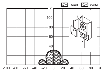
V680-HS61 (embedded in non-metallic material) & V680-D1KP66MT (mounted on metallic surface: steel)
