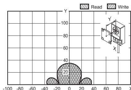
V680-HS65 (mounted on metallic material) & V680S-D2KF67M (mounted on metallic surface: steel)
