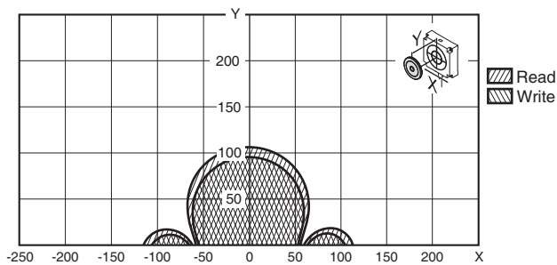
High-temperature Type 1-kbyte Memory RF Tags V680-HS65 (with metal on back surface) & V680-D1KP58HTN
