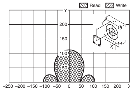
V680-HS65 (mounted on metallic material) & V680S-D2KF67 (mounted on non-metallic material)
