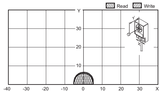
V680-HS61 (mounted on non-metallic material) & V680-D1KP52MT (embedded in metallic surface: steel)
