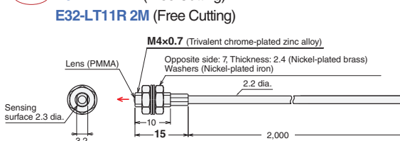
29-C E32-LT11 2M (Free Cutting)
