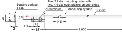
17-A E32-T15XR 2M (Free Cutting)
