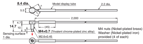
11-B E32-T11N 2M (Free Cutting)
