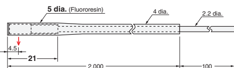
43-D E32-T14F 2M (Free Cutting)
