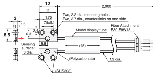
17-G E32-LT35Z 2M (Free Cutting)
