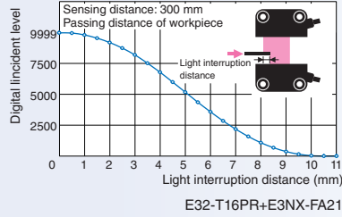
Characteristics of Light Interruption (Reference Value)
