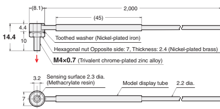
11-A E32-LT11N 2M (Free Cutting)
