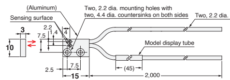
19-E E32-D15ZR 2M (Free Cutting)
