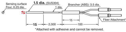
Enlarged View of Sensing Surface
