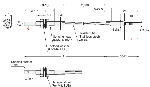
49-F E32-T64-2 2M (No Cutting)
