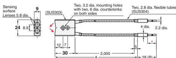
51-G E32-A09H2 2M (No Cutting)
