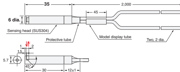
15-G E32-D14LR 2M (Free Cutting)
