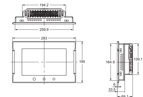
Cable Connection Dimensions
