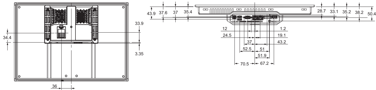
Cable Connection Dimensions
