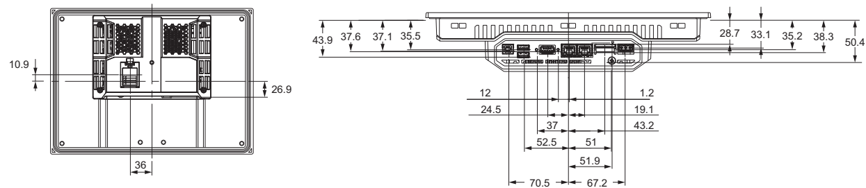
Cable Connection Dimensions
