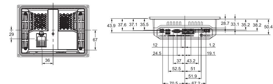
Cable Connection Dimensions
