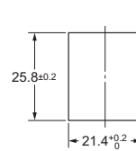
Mounting Hole Dimensions
