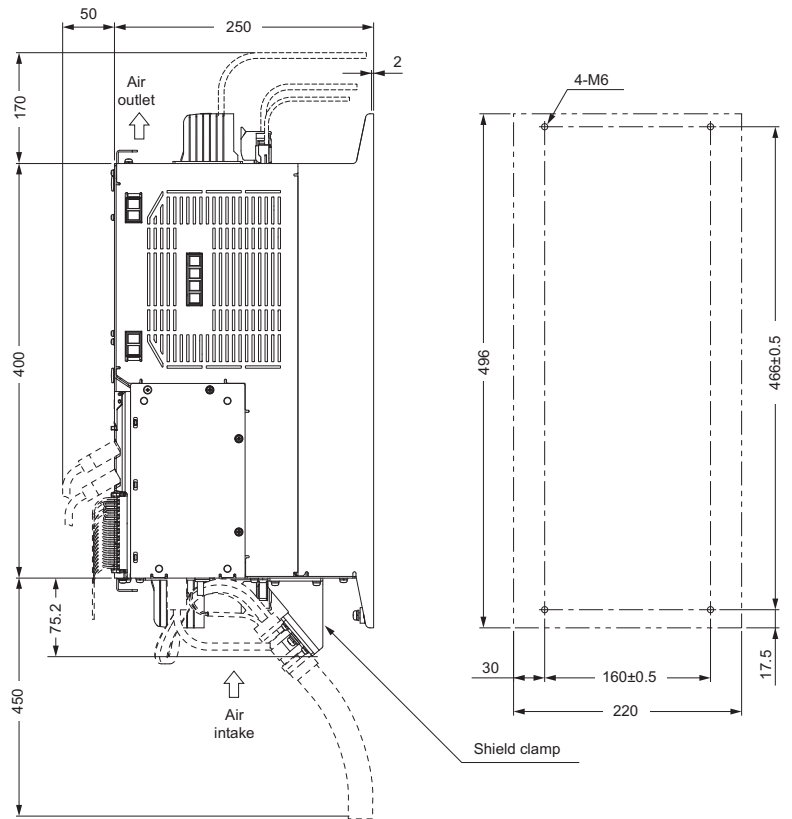
Mounting dimensions
