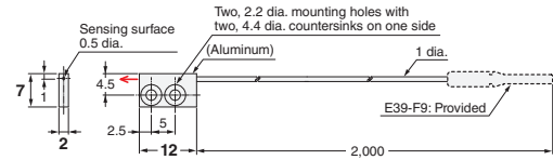
45-D E32-T25XB 2M (Free Cutting)
