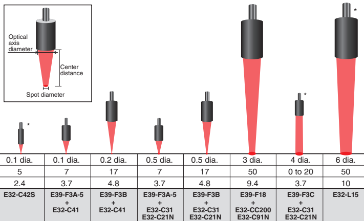
<Map of Spot Diameters and Center Distances>
