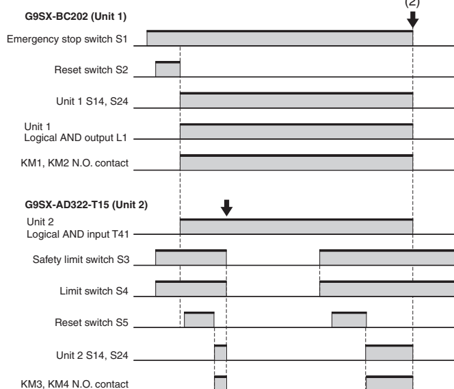
Timing chart 1
