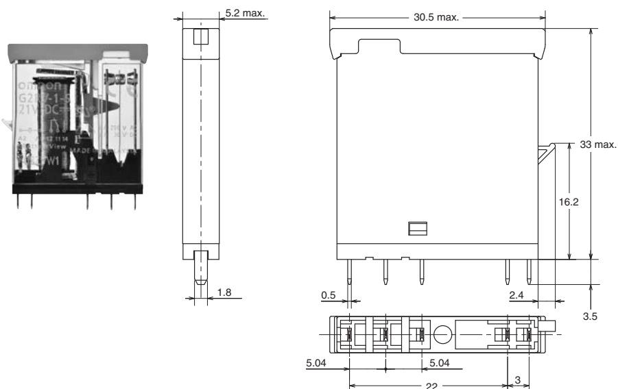
Terminal Arrangement/ Internal Connection Diagram (TOP VIEW)
