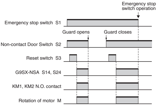
Timing chart
