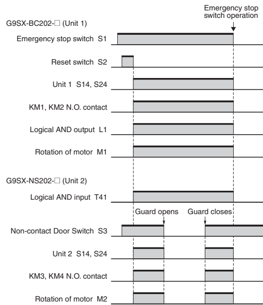
Timing chart
