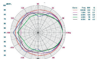
Circular chart of directional characteristic:
