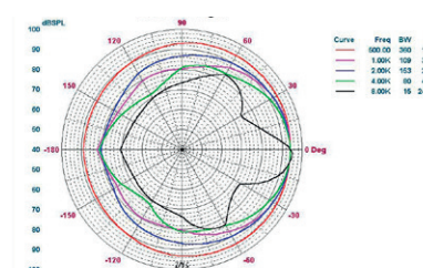
Circular chart of directional characteristic:
