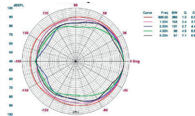
Circular chart of directional characteristic:
