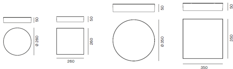
ICR26 – 20W
