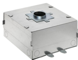
WC3105 Solid walls outer casing Cassaforma per muratura
