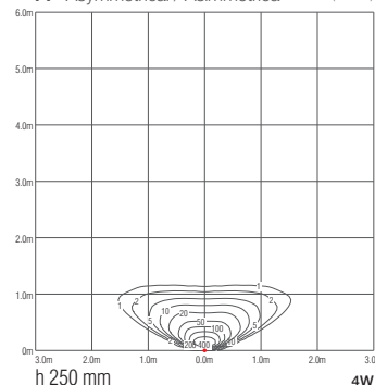
A - Asymmetrical / Asimmetrica Isolux (3000K)
