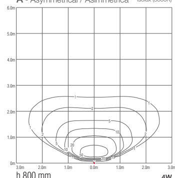
A - Asymmetrical / Asimmetrica Isolux (3000K)
