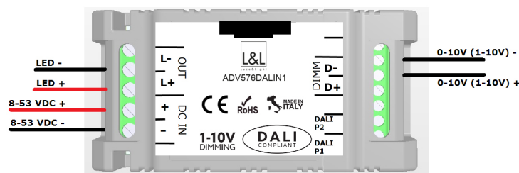
Collegamento 0-10V (fig. 4) / 0-10V connection (pic. 4)
