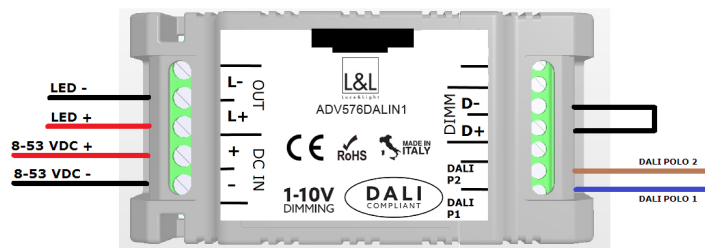
Collegamento DALI (fig. 6) / DALI connection (pic. 6)
