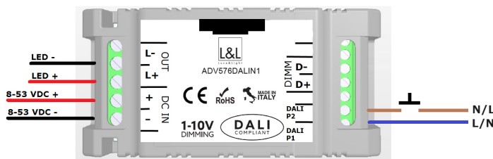
Collegamento pulsante (fig. 5) / Push button connection (pic. 5)
