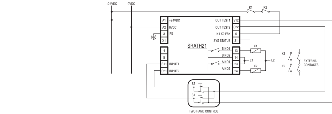
Automatic mode with K1 K2 FBK control
