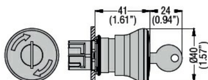
Turn key to release
