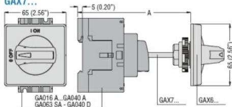
Shaft extensions for door coupling handles GAX7...
